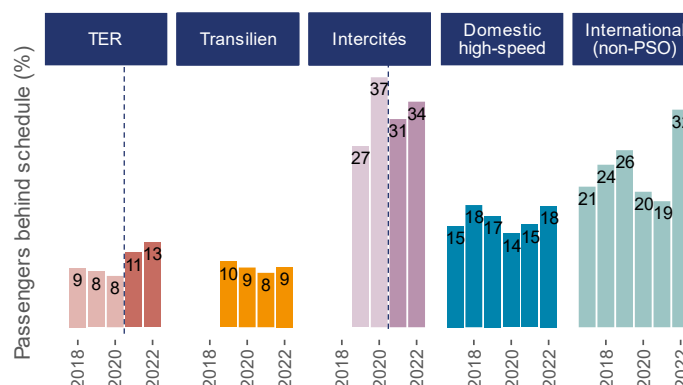
Figure 36 – Proportion of passengers behind schedule at destination (5min threshold)
